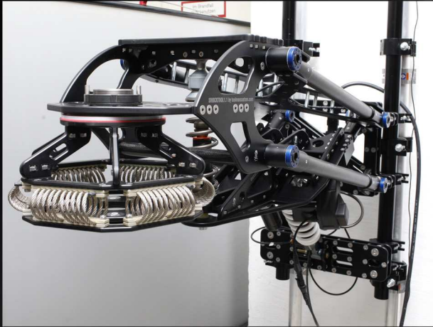
shocktool shown with our springmount
